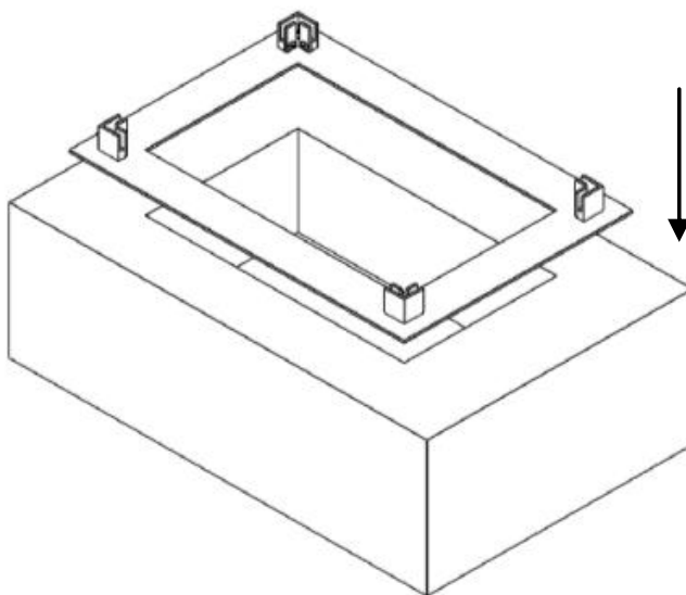
Figure 2 —Placing the support in the installation hole
