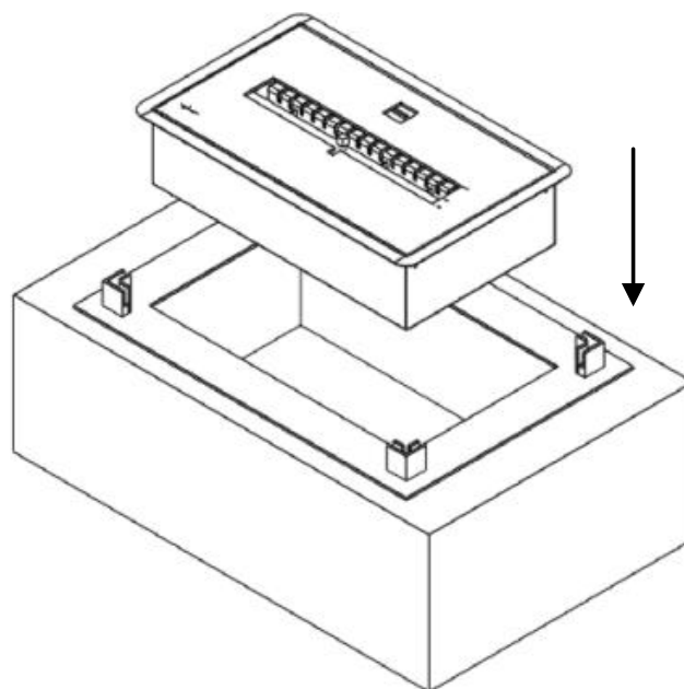
Figure 3 —Placing the Burner II on the support
