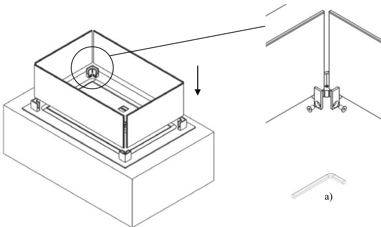
Figure 4 —Installation of protection glasses
