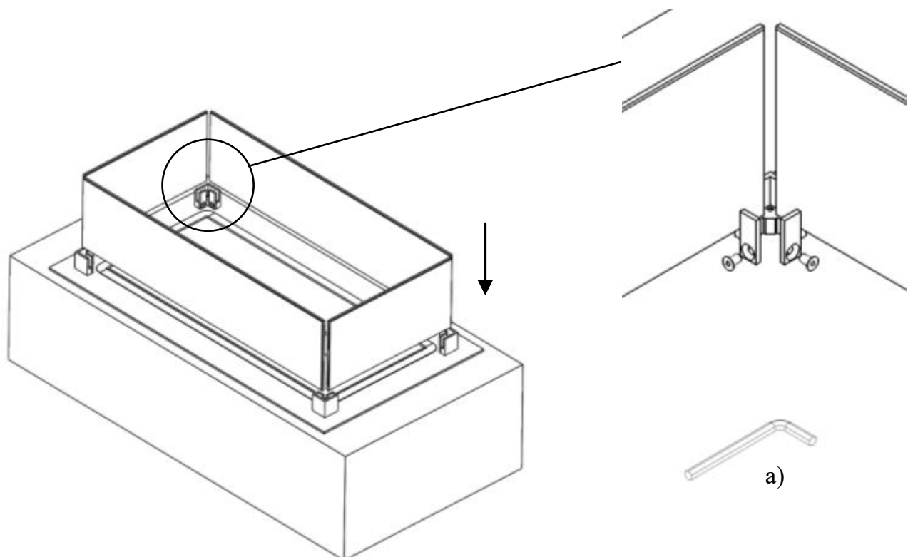
Figure 4 —Installation of protection glasses
